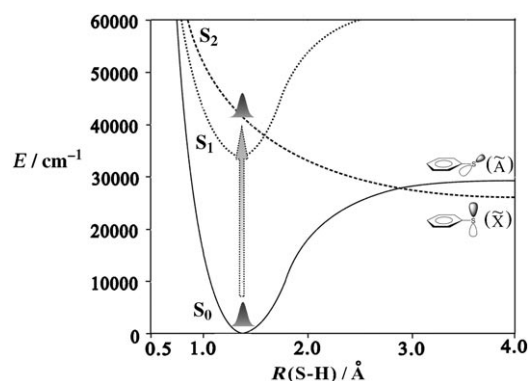
Figure 1. Diabatic potential-energy surfaces of thiophenol along the S–H bond elongation coordinate at planar geometry. At 243 nm, the wavepacket is exclusively prepared on S_2 .
